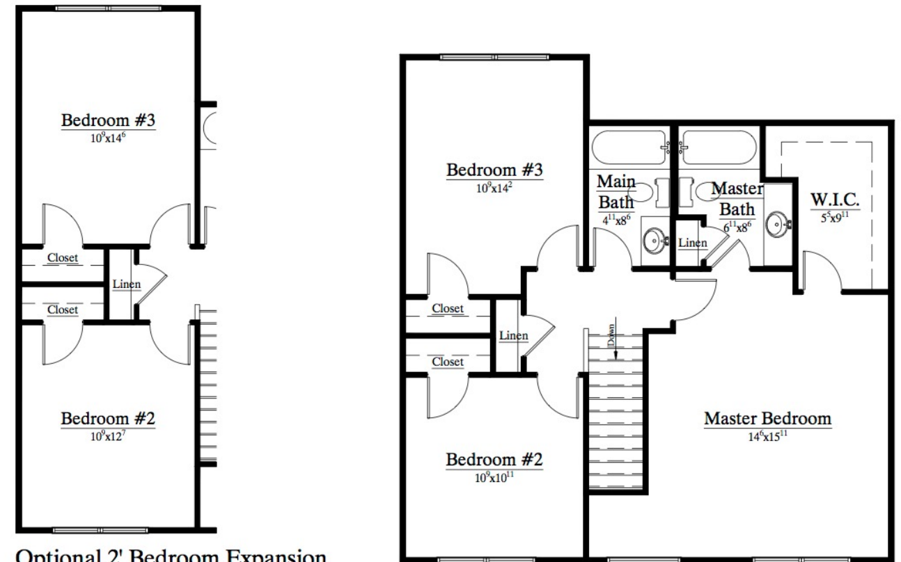
Optional 2' Bedroom Expansion w/ Optional 2' Dinette Expansion (Rear of Dinette and Bedroom #3)
