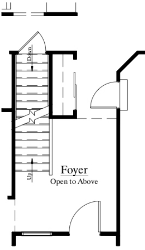
First Floor w/ Optional Loft or Bedroom
