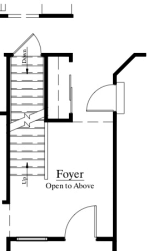
First Floor w/ Optional Loft or Bedroom
