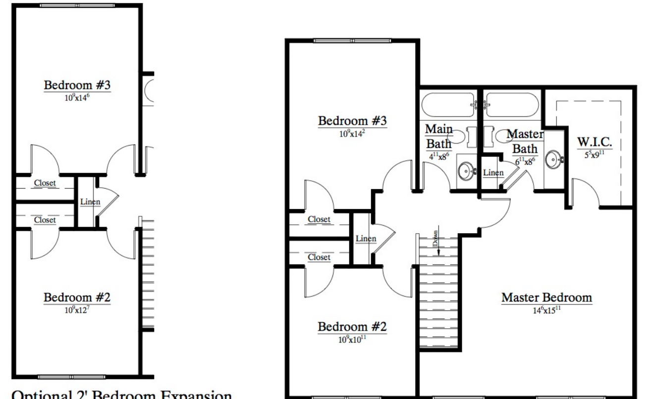
Optional 2' Bedroom Expansion w/ Optional 2' Dinette Expansion (Rear of Dinette and Bedroom #3)
